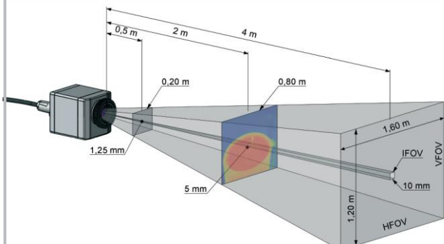
Measurement field of the thermal imager PSC PI as an example with the standard lens 23° x 17°
